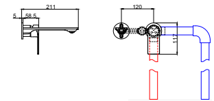
DG507-DYH 暗装面盆龙头 Concealed basin mixer
