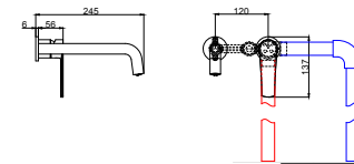
DG504 暗装面盆龙头 Concealed basin mixer
